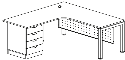
L SHAPE TABLE C/W FIXED 4D ( L ) MUMD-8286 L1800/750 x W1800/600 x H750 MUMD-8656 L1800/600 x W1800/600 x H750 MUMD-5656 L1500/600 x W1500/600 x H750
