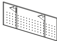
METAL MODESTY PANEL c/w BRACKET MUMP 1800 L1600 x W20 x H450 MUMP 1500 L1300 x W20 x H450 MUMP 1200 L1000 x W20 x H450
