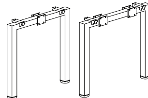
N LEG (MIDDLE) MUN1800(M) L1790 x H725 MUN1500(M) L1490 x H725 MUN1200(M) L1190 x H725 MUN1050(M) L1040 x H725 MUN 900(M) L890 x H725 MUN 750(M) L740 x H725 MUN 600(M) L590 x H725
