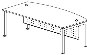
EXECUTIVE TABLE (D-SHAPE) MUME-1890 L1800 x W900/750 x H750
