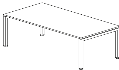
RECTANGULAR CONFERENCE TABLE MUC-4815 L4800 x W1500 x H750 MUC-3615 L3600 x W1500 x H750 MUC-3012 L3000 x W1200 x H750 MUC-2412 L2400 x W1200 x H750 MUC-2010 L2100 x W1050 x H750 MUC-1890 L1800 x W900 x H750
