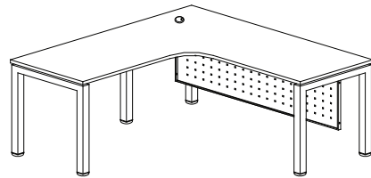
L SHAPE TABLE ( L ) MUML-8286 L1800/750 x W1800/600 x H750 MUML-8656 L1800/600 x W1800/600 x H750 MUML-5656 L1500/600 x W1500/600 x H750
