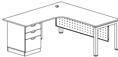
L SHAPE TABLE C/W FIXED 2D1F ( L ) MUMF-8286 L1800/750 x W1800/600 x H750 MUMF-8656 L1800/600 x W1800/600 x H750 MUMF-5656 L1500/600 x W1500/600 x H750
