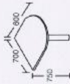
RE-HRCT70 Half Round Connection Top with Metal Leg L600 x W700 x H750
